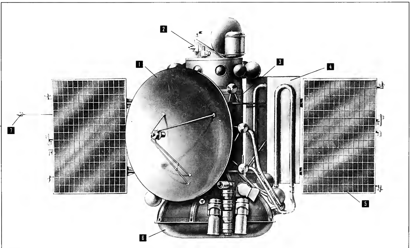
Figure 18. The Mars 4 and 5 Spacecraft—(1) high-gain antenna, (2) radiometer, (3) fuel tank, (4) radiators of the temperature control system, (5) solar panel, (6) instrument module, and (7) magne- tometer
